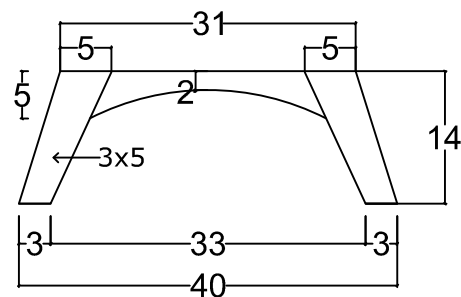
FRONT VIEW T. Depan
