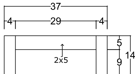
SIDE VIEW T. Samping
