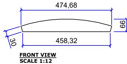
FRAME MIRROR 3 Qty : 1 pcs
