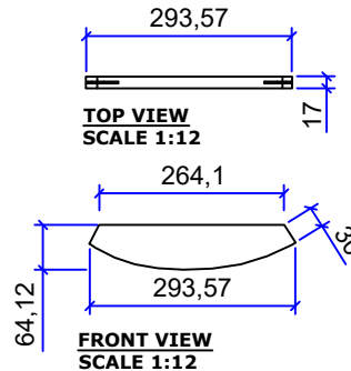
FRAME MIRROR 6 Qty : 1 pcs
