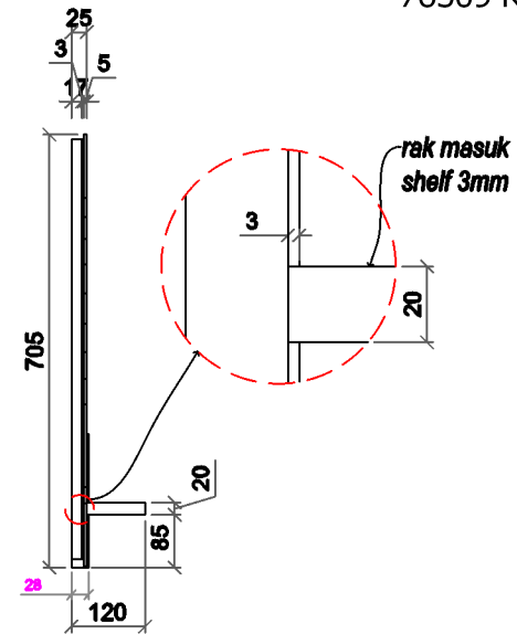
SIDE VIEW T.Samping
