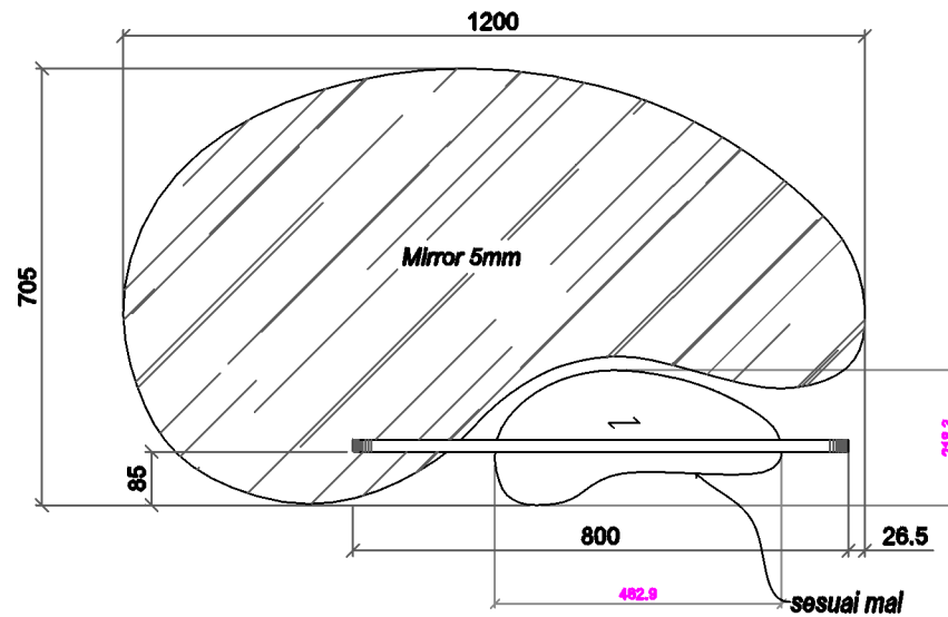
FRONT VIEW T.Depan
