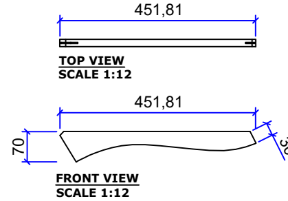
FRAME MIRROR 6 Qty : 1 pcs
