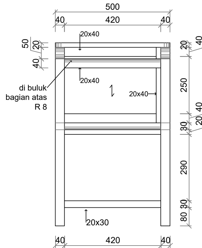
T. SAMPING KIRI SCALE 1:10
