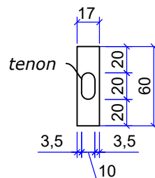
SIDE VIEW SCALE 1:4
