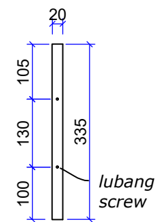
SIDE VIEW SCALE 1:10
