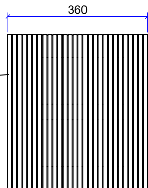
FRONT VIEW SCALE 1:10
