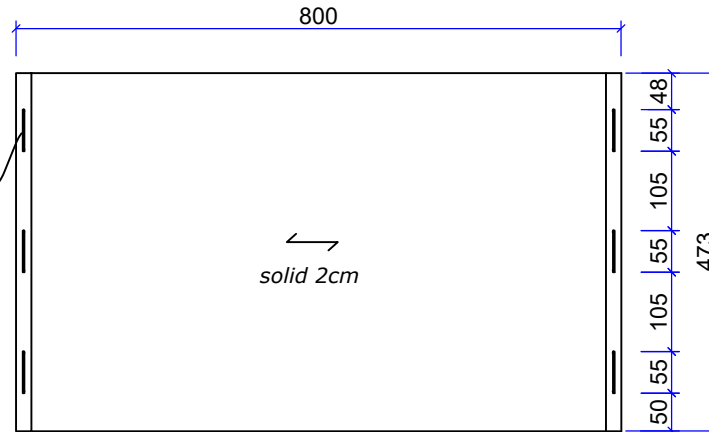
BOTTOM VIEW SCALE 1:10
