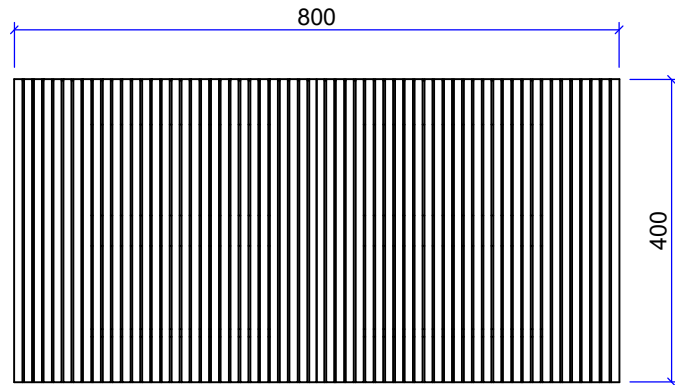
FRONT VIEW SCALE 1:10
