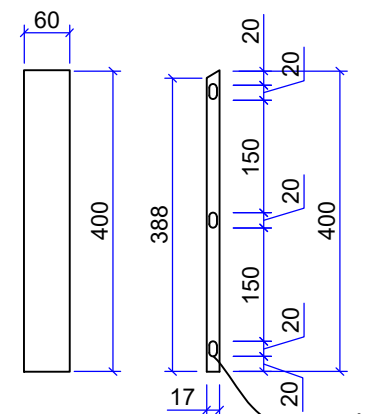
FRONT VIEW SCALE 1:10
