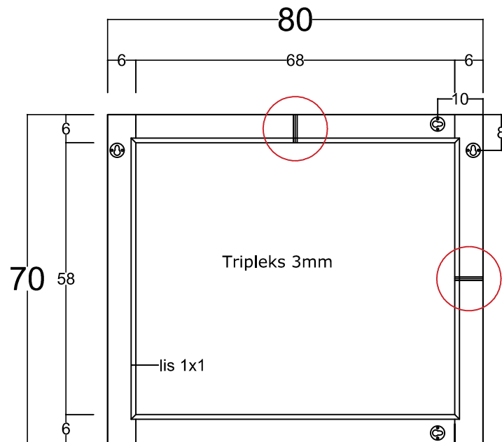
REAR VIEW T.Belakang
