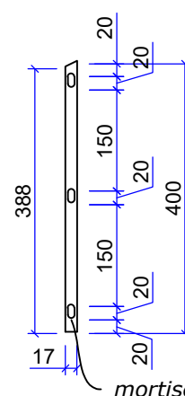
SIDE VIEW SCALE 1:10
