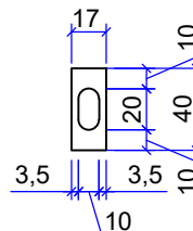
SIDE VIEW SCALE 1:4
