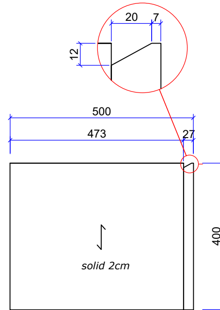
SIDE VIEW SCALE 1:10
