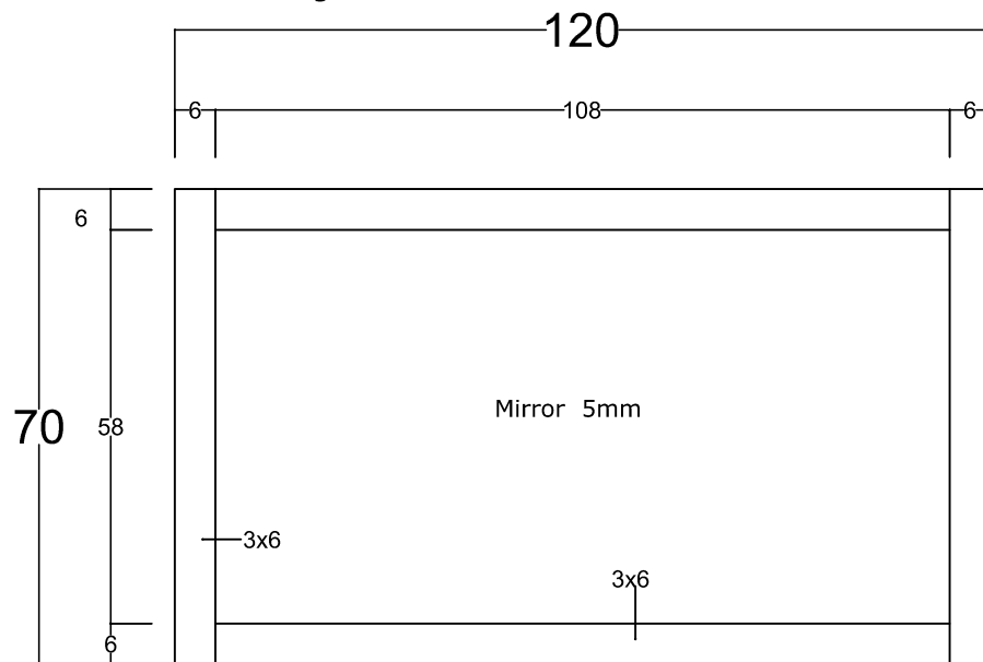
REAR VIEW T.Belakang
