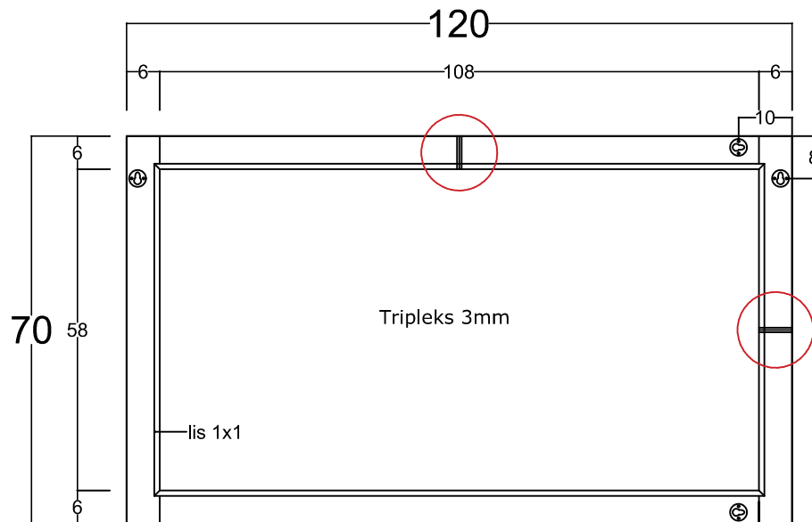
REAR VIEW T.Belakang
