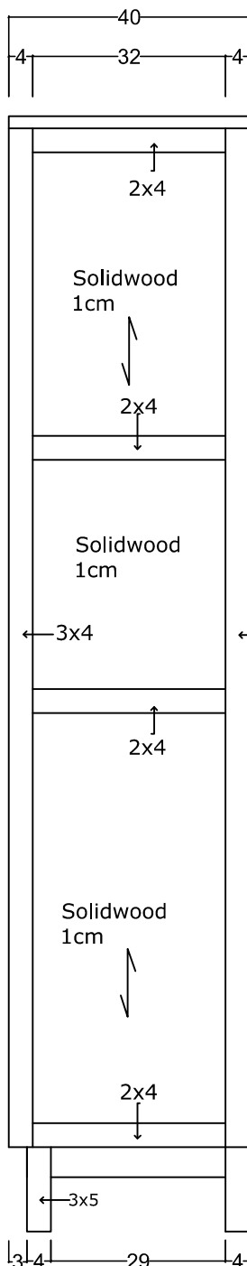
SIDE VIEW T. Samping
