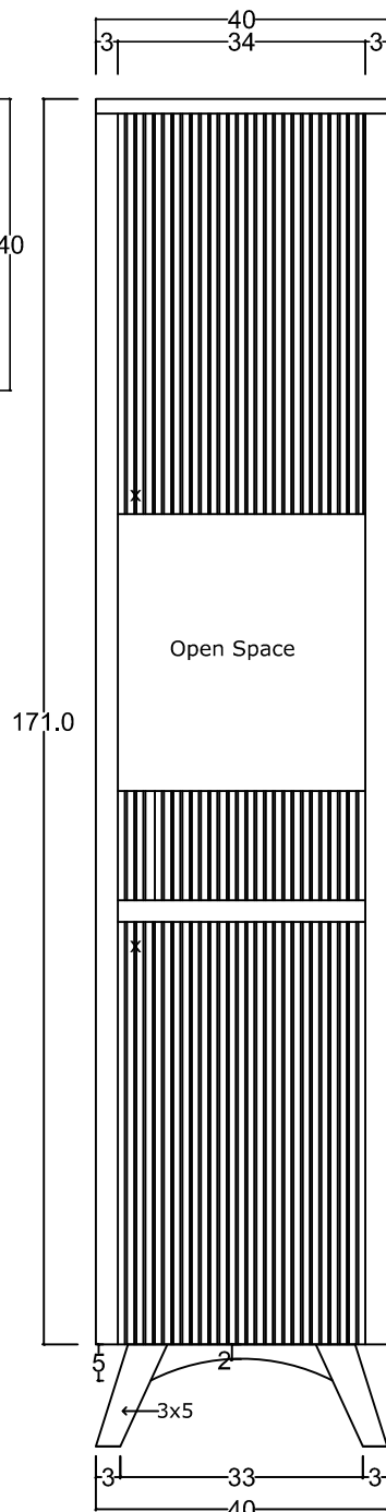
FRONT VIEW T. Depan
