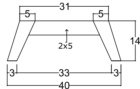
REAR VIEW T. Belakang
