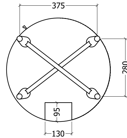
BOTTOM VIEW SCALE 1:12
