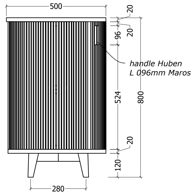
SIDE VIEW SCALE 1:12
