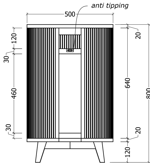
BACK VIEW SCALE 1:12
